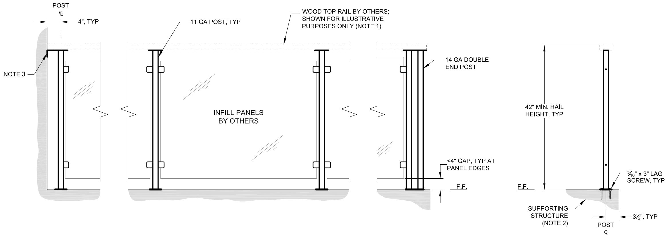
1 END POST - WALL CONNECTION ELEVATION SCALE: NONE
